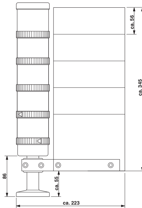
Dimensional drawing
